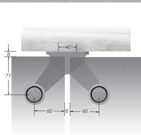
VISTA FRONTAL (6192)
